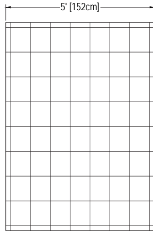
3-PIECE PANEL DIMENSIONS
