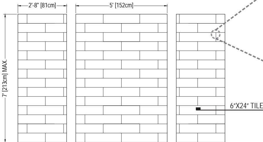
3-PIECE PANEL DIMENSIONS
