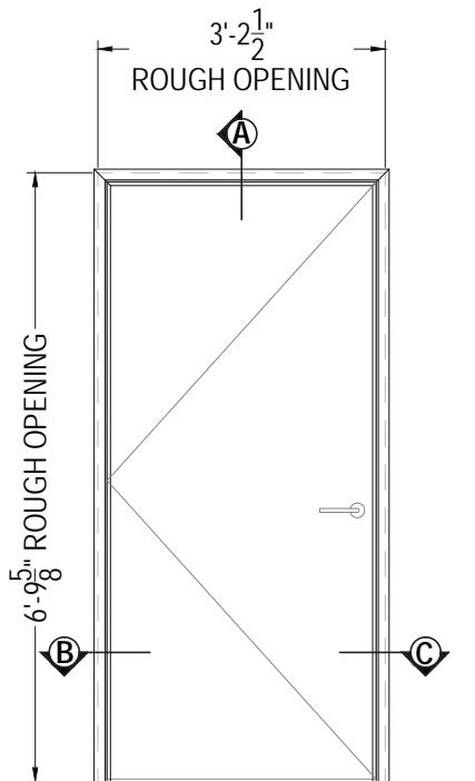
3/0 X 6/8 TIMELY 18GA DOOR FRAME
