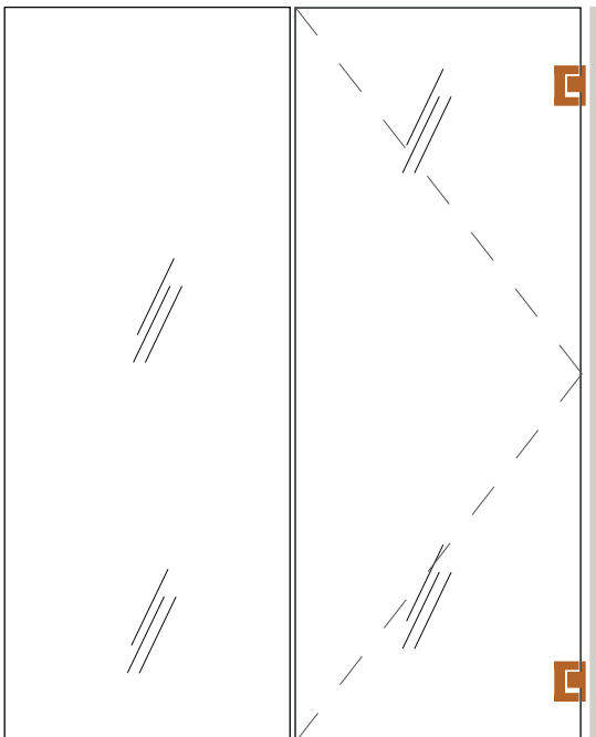
GLASS-TO-WALL HINGE W/ FIXED PANEL AT STRIKE SIDE
